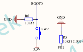
BOOT
