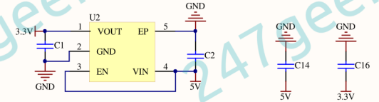
5V -> 3.3V
